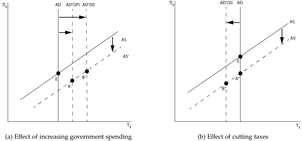
Figure 1: Policy predictions of ZLB-EX
